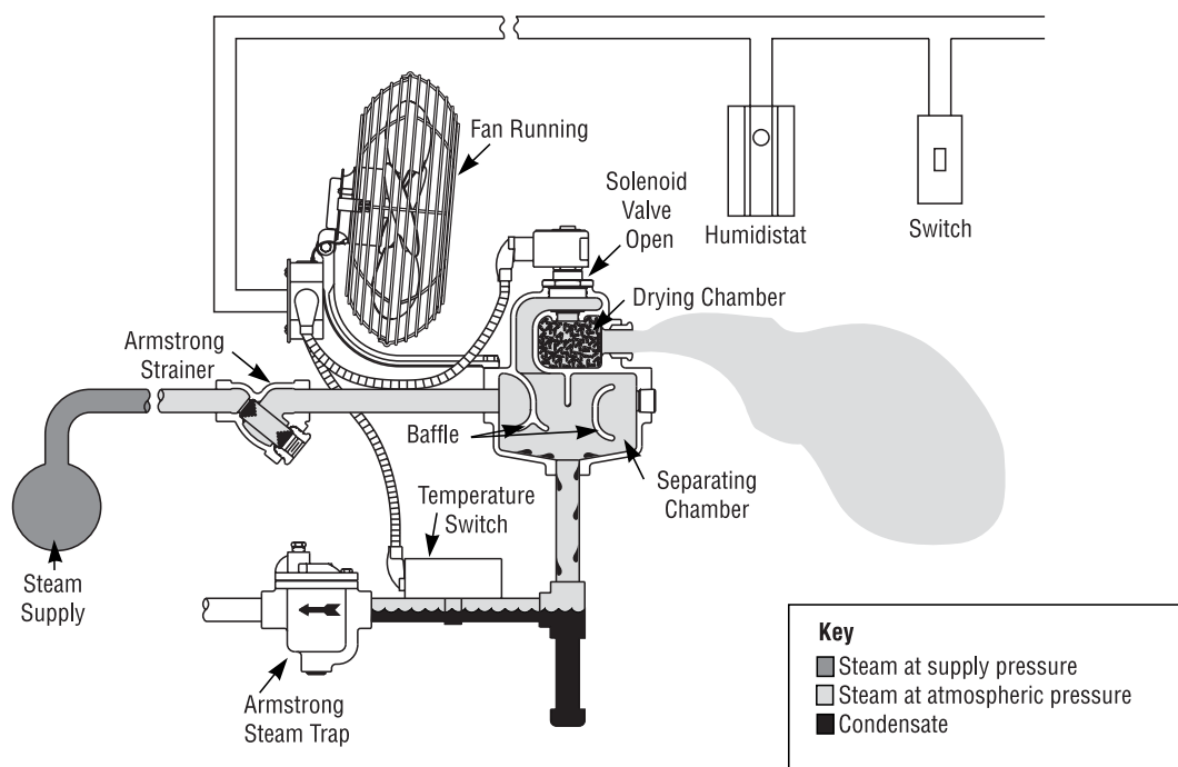
Figure 60-1. How Armstrong Conditioned Steam Humidifiers Operate for Area Humidification
