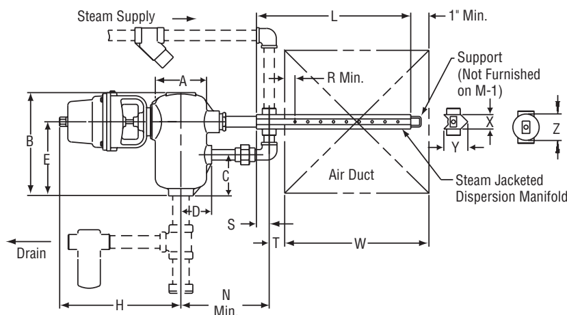
Figure 72-1. Dimensions
